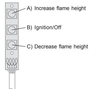
Figure 5: Switch Panel
