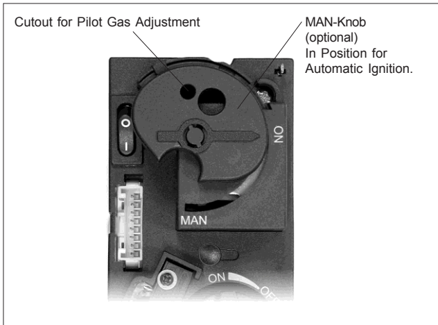
Figure 3: Combination Control, View MAN-Knob (optional)
