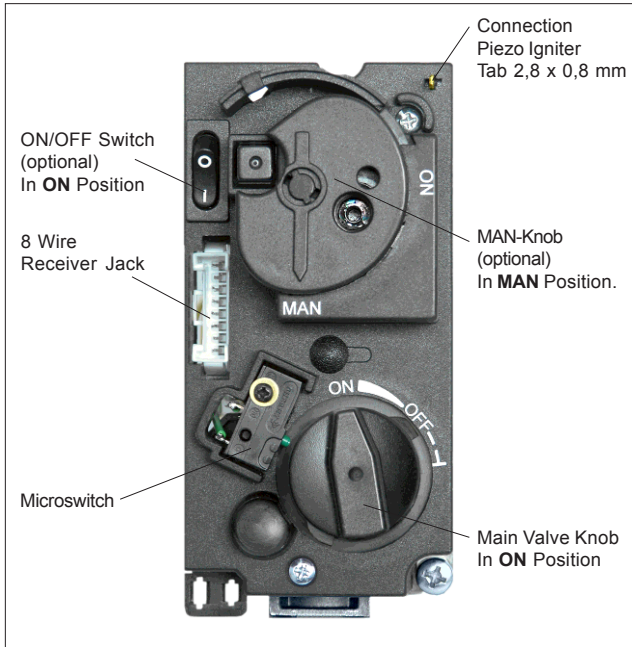
Figure 2: Combination Control, Cover
